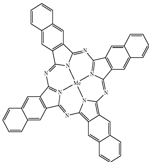
[Naphthalocyanine]
