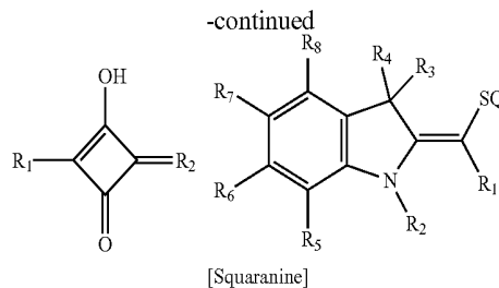
[Squaraine]
