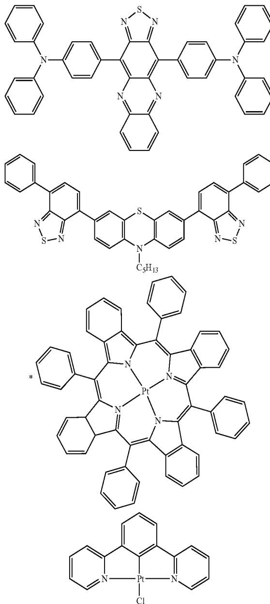
[Chemical Formula 1]
